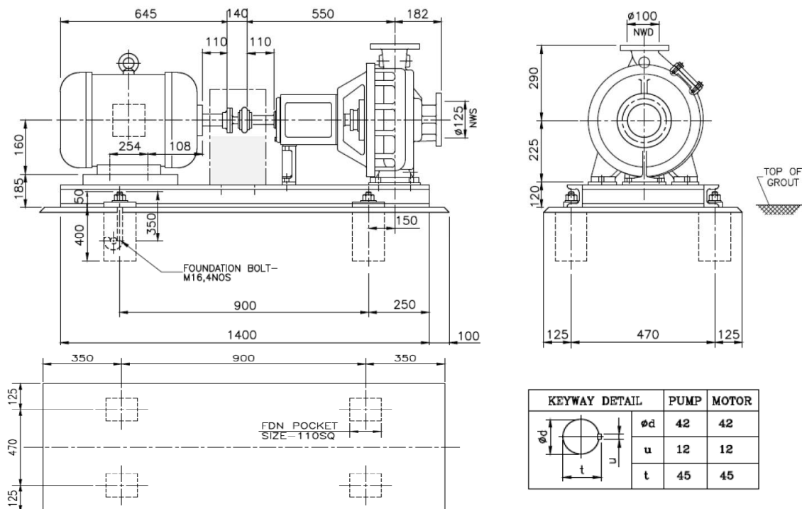
Horizontal Centrifugal Non-clogging Pump General Arrangement
